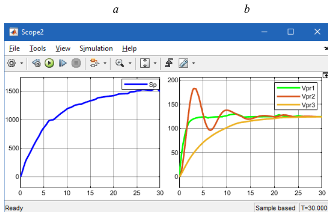
Fig. 10. An FLC in modeling the mill control system for the first-stage grinding ore: a - pulp density in a mill, b - consumption of crushed ore at the outlet of the mill
